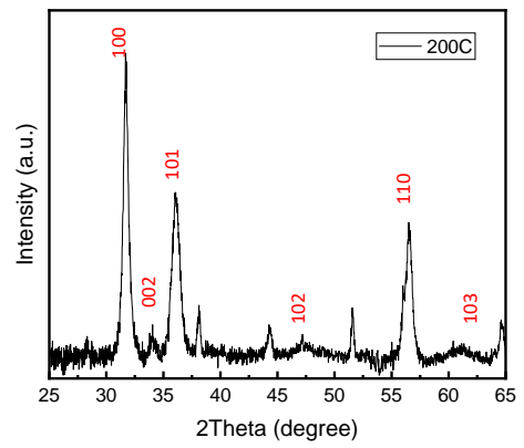
Figure 2 XRD pattern of ZnO
