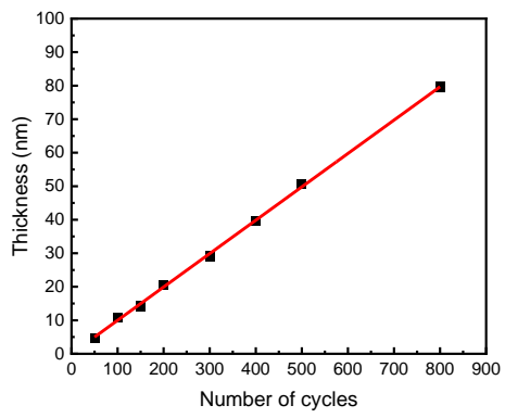
Figure 1 Thickness vs number of cycles
