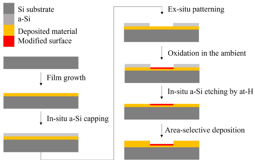
Figure 1: Schematic representation of the chemical patterning and area-selective deposition process.
