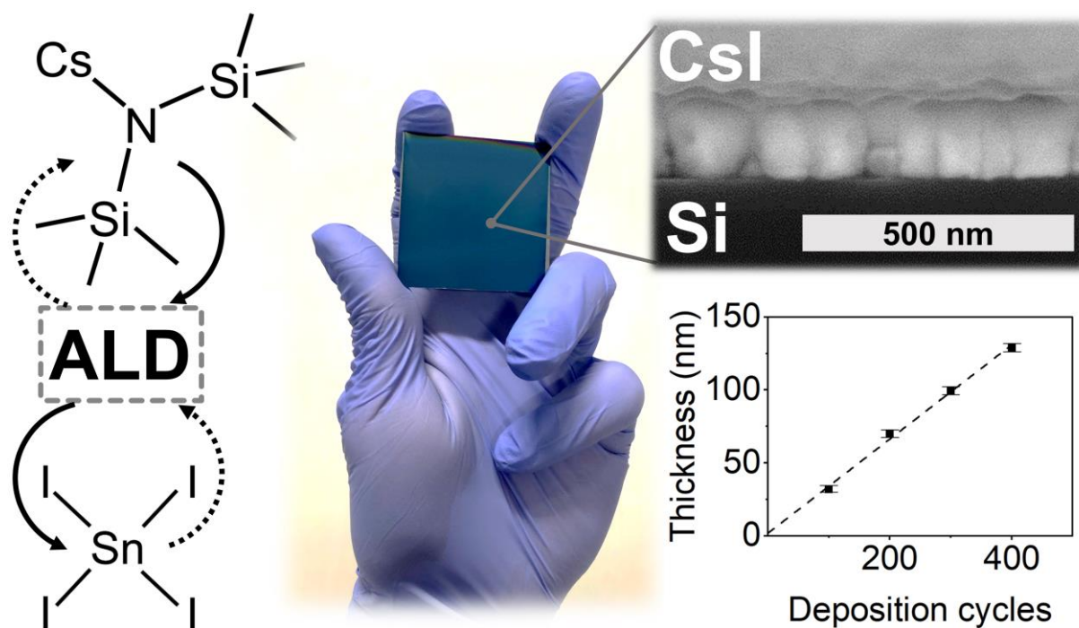
Figure 1: Left: Structures of the precursors. Middle: ALD CsI film deposited on silicon substrate. Right-top: FESEM cross-sectional image of the same film. Right-bottom: Film thickness over CsI deposition cycles.
