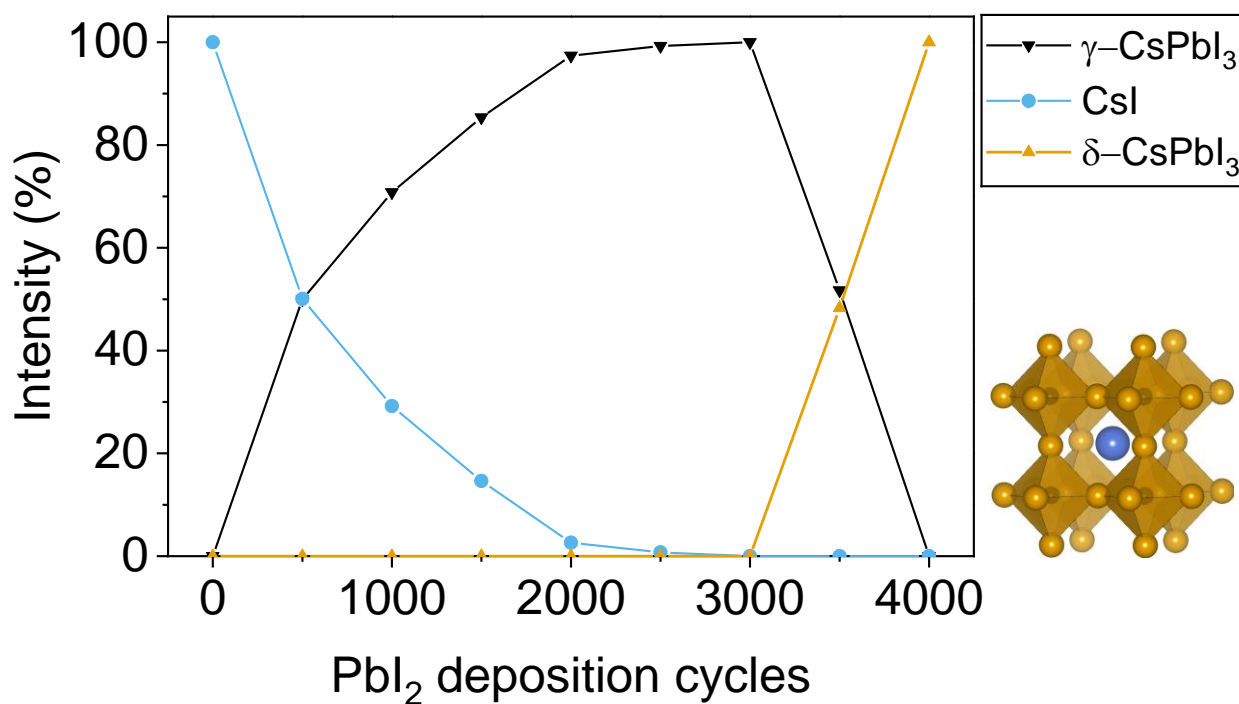
Figure 2: Relative intensity (area, counts times degrees of 2 \theta ) of different phases as a function of PbI 2 deposition cycles on the CsI thin film.
