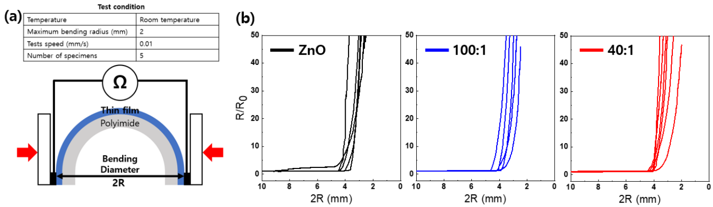
Supporting 2 (a) Test conditions for thin film bending (b) Bending test results of ZnO-HQ thin films
