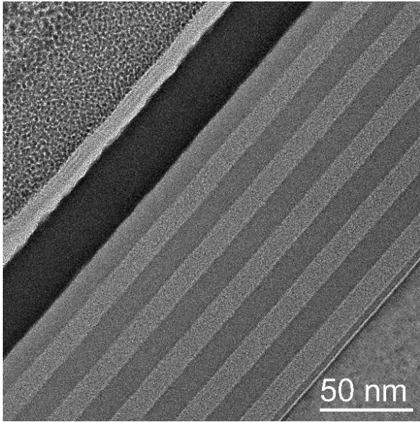
Figure 1: HR-TEM image of an ALD/MLD-multilayer
