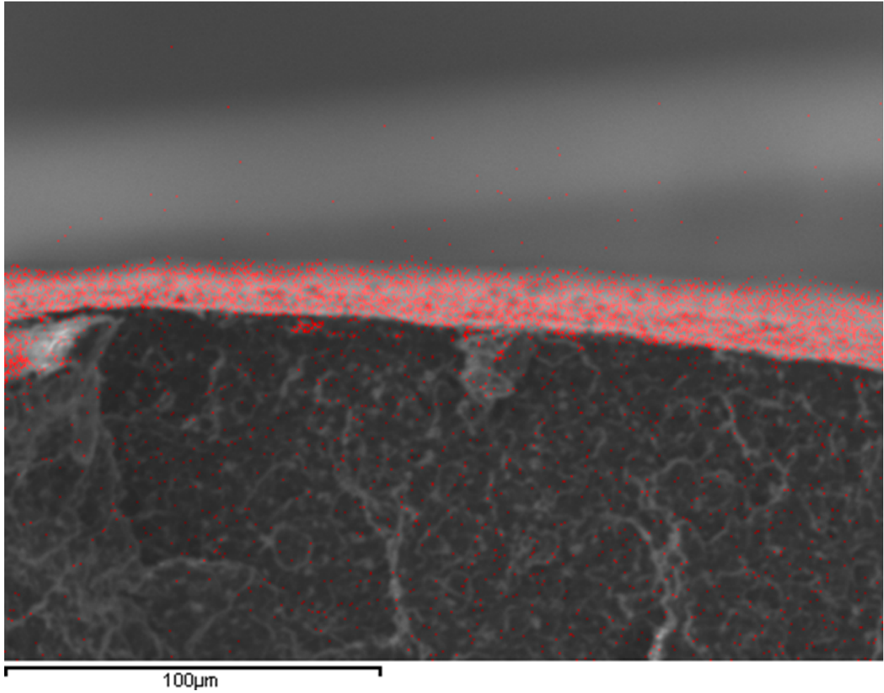
Figure 1. EDS mappings of aluminum content overlaid on SEM images of ABS polymer cross sections after deposition of Alumina by ALD. Red dots indicated aluminum concentration..
