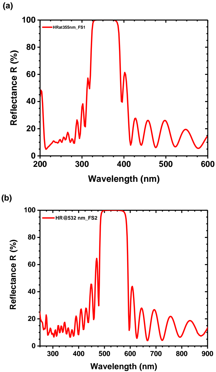
Fig. 1 Reflectance spectra of HfO 2 /SiO 2 multilayer at (a) 355 nm and (b) 532 nm wavelength.
