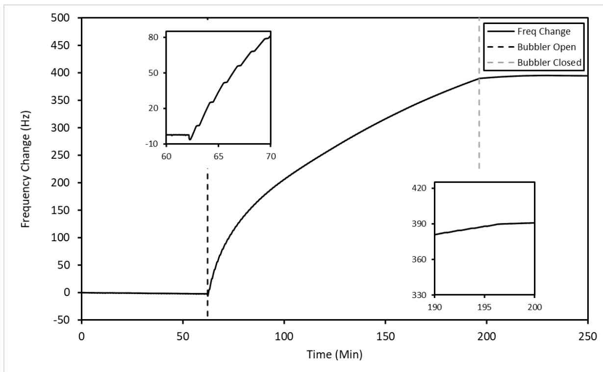
Figure 1. A quartz crystal microbalance (QCM) trace of the change in frequency (where higher frequency \sim lower mass) with increasing exposure to the novel precursor 1,3-diisopropylimidazol-2-ylidene)methylgold(I). The insets show the slope of the etch at the beginning and end of the process.
