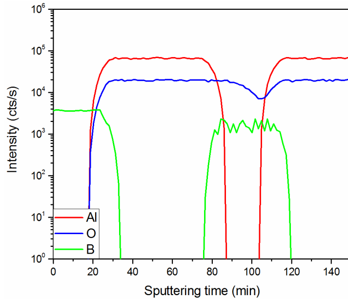
SIMS measurements of the heterostructure BN/Al 2 O 3 -ALD/BN/Al 2 O 3
