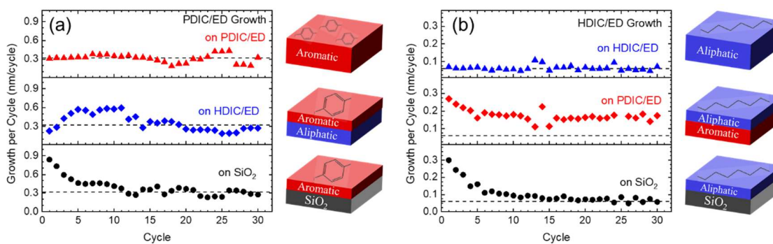
Figure 2. Growth per cycle for (a) PDIC/ED and (b) HDIC/ED deposited on various substrates: SiO 2 (black), PDIC/ED (red), and HDIC/ED (blue). Steady growth rates on SiO 2 are indicated by horizontal dashed lines for reference.
