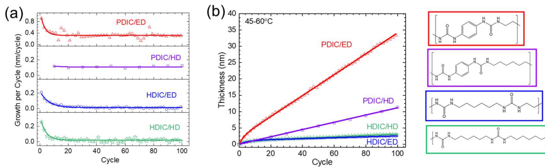
Figure 1. Experimental data (points) and model fit (solid line) for PDIC/ED (red), PDIC/HD (purple), HDIC/ED (blue) and HDIC/HD (green) films, showing (a) growth rate and (b) thickness vs cycle number for all films.
