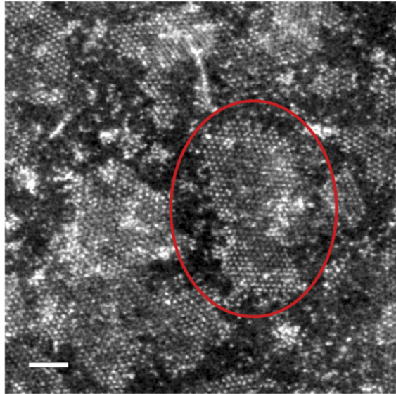
(left) 2D \text{MoS}_2\text{-WSe}_2 core-shell quantum dot grown by PEALD, imaged with HAADF-STEM. Scale bar: 2 nm. (right) Numerical simulation of the core-shell growth, highlighting the importance of reactive edge sites in the formation of these structures.
