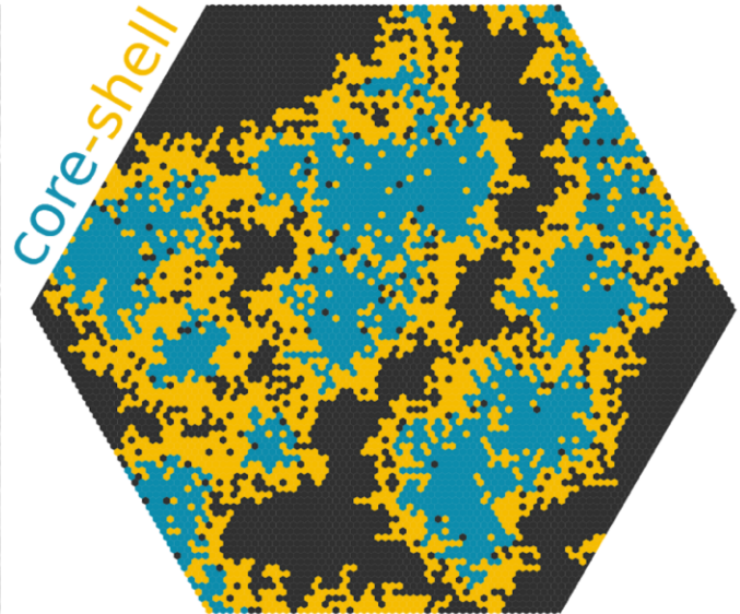
(left) 2D \text{MoS}_2\text{-WSe}_2 core-shell quantum dot grown by PEALD, imaged with HAADF-STEM. Scale bar: 2 nm. (right) Numerical simulation of the core-shell growth, highlighting the importance of reactive edge sites in the formation of these structures.
