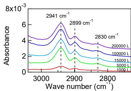
Fig. 1. IR absorbance spectra measured from the TMA adsorbed surfaces at 160 °C.
