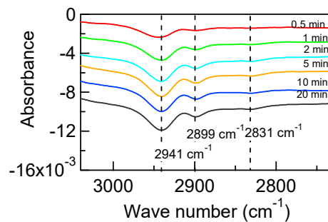
Fig. 2. IR absorbance spectra measured from the TMA adsorbed surfaces at 160 °C with plasma-excited \text{NH}_3 treatments.
