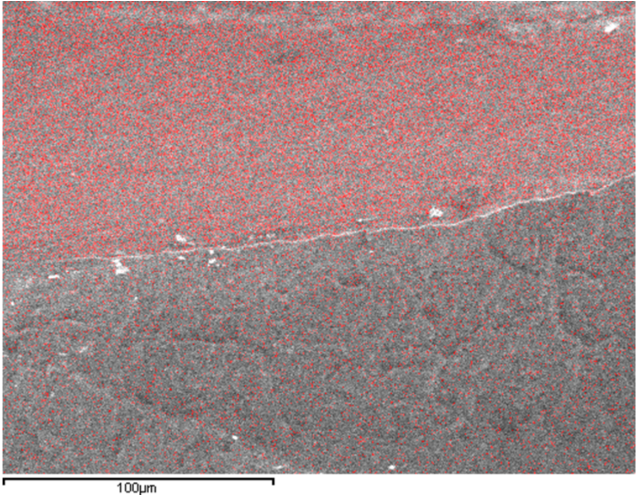
Figure 1. SEM cross sectional view of 3D printed ABS polymer coated with alumina by ALD, overlaid with EDX mapping of Al concentration shown in red.
