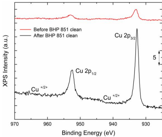
e) HR-XPS of Cu 2p region after thiol removal
