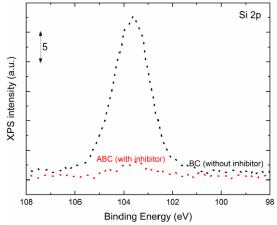
f) HR-XPS of Si 2p region after thiol removal
