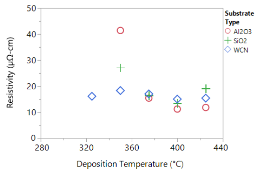
Fig. 1. Resistivity of Ir and IrOx films by ALD at 325-425°C using (MeCp)Ir(COD) and O 2
