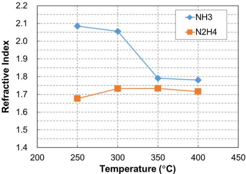
Fig. 3. Deposition temperature dependence of R.I..
