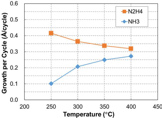
Fig. 2. Deposition temperature dependence of GPC.
