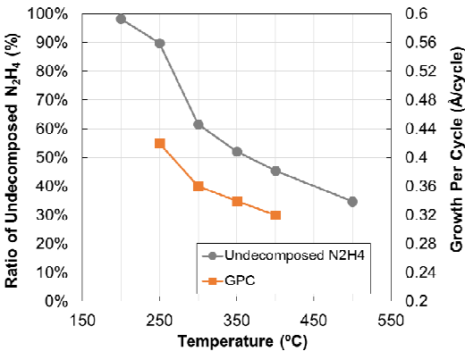
Fig. 1. Ratio of undecomposed N2H4 and GPC for temperature.
