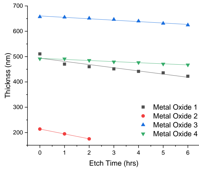
Figure 1. Film thickness loss as a function of etch time comparison of 4 plasma-resistant films.
