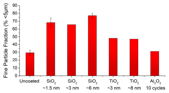
Figure 1: In-vitro dissolution profiles and fine particle fractions of uncoated and ALD-coated budesonide with different shell thicknesses of Al 2 O 3 , TiO 2 and SiO 2 .
