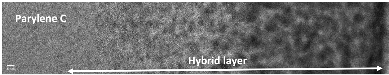
Fig.1. TEM micrograph of lamellae of paryleneC modified with indium oxide by VPI.
