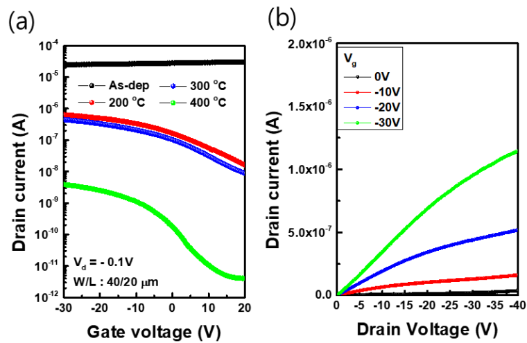
Figure 1. Transfer characteristic with drain voltage of -0.1 V (a), and output curve (b) of SnO TFTs
