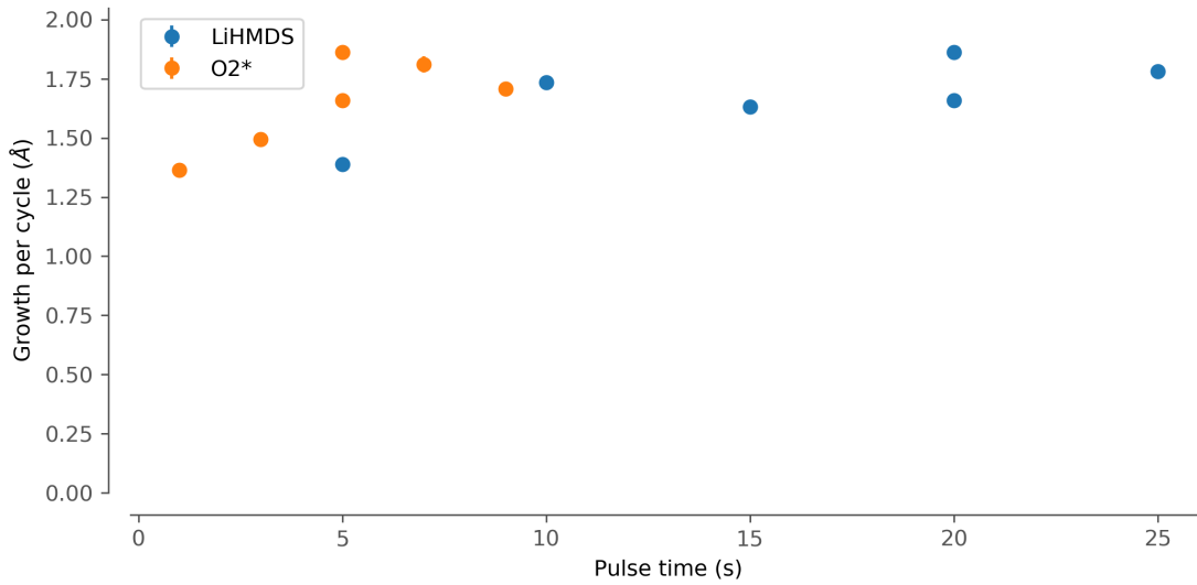
Fig. 1 Saturation curves for the lithium silicate process, deposited at 150°C.
