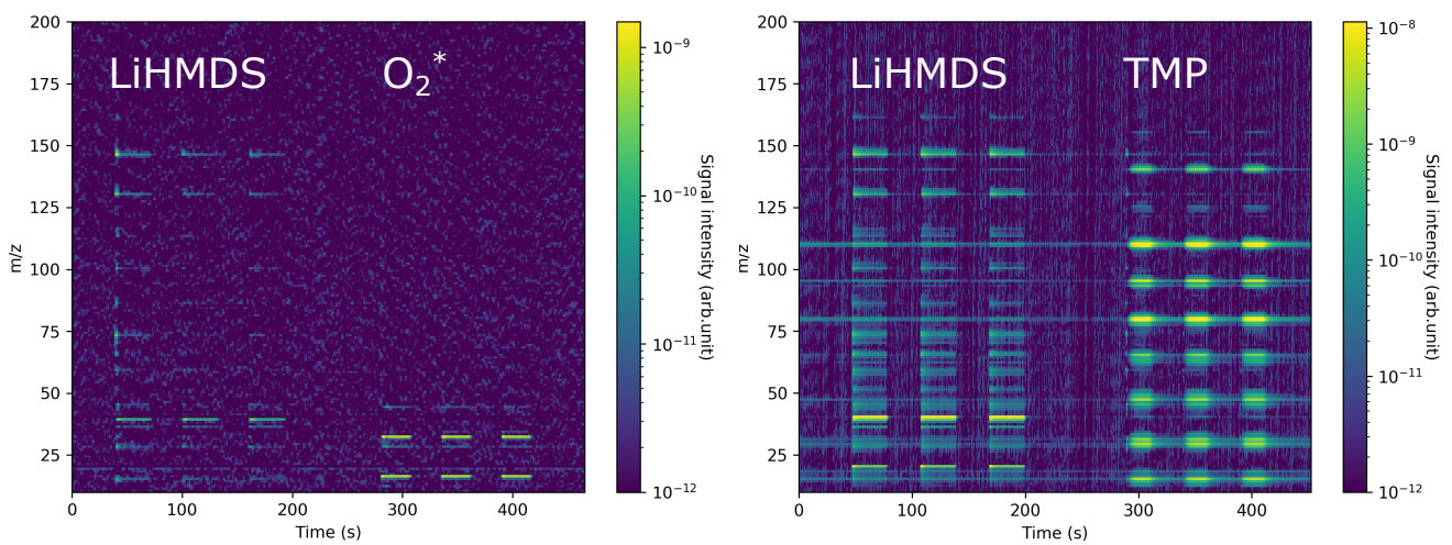
Fig. 3 Mass spectrometry results for LiHMDS-O 2 * process (left) and LiHMDS-TMP process (right)
