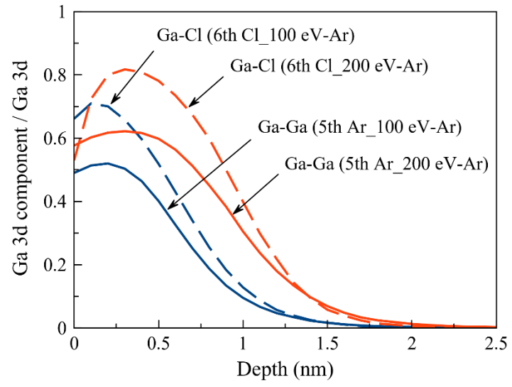
Fig.1 Depth profiles of Ga-Ga and Ga-Cl bond concentration estimated by angle resolved XPS
