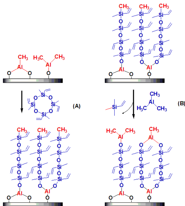
Figure 1. Reaction scheme for V_4D_4/TMA MLD
