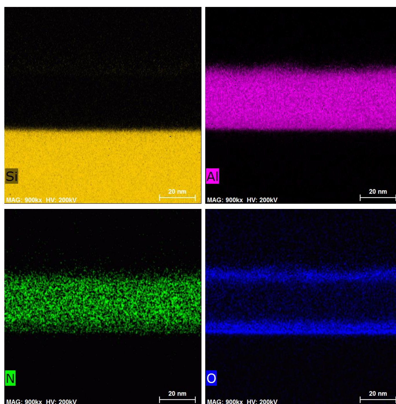
Figure 3. Cross-sectional EDS mapping data of ALD AlN film on Si(100).
