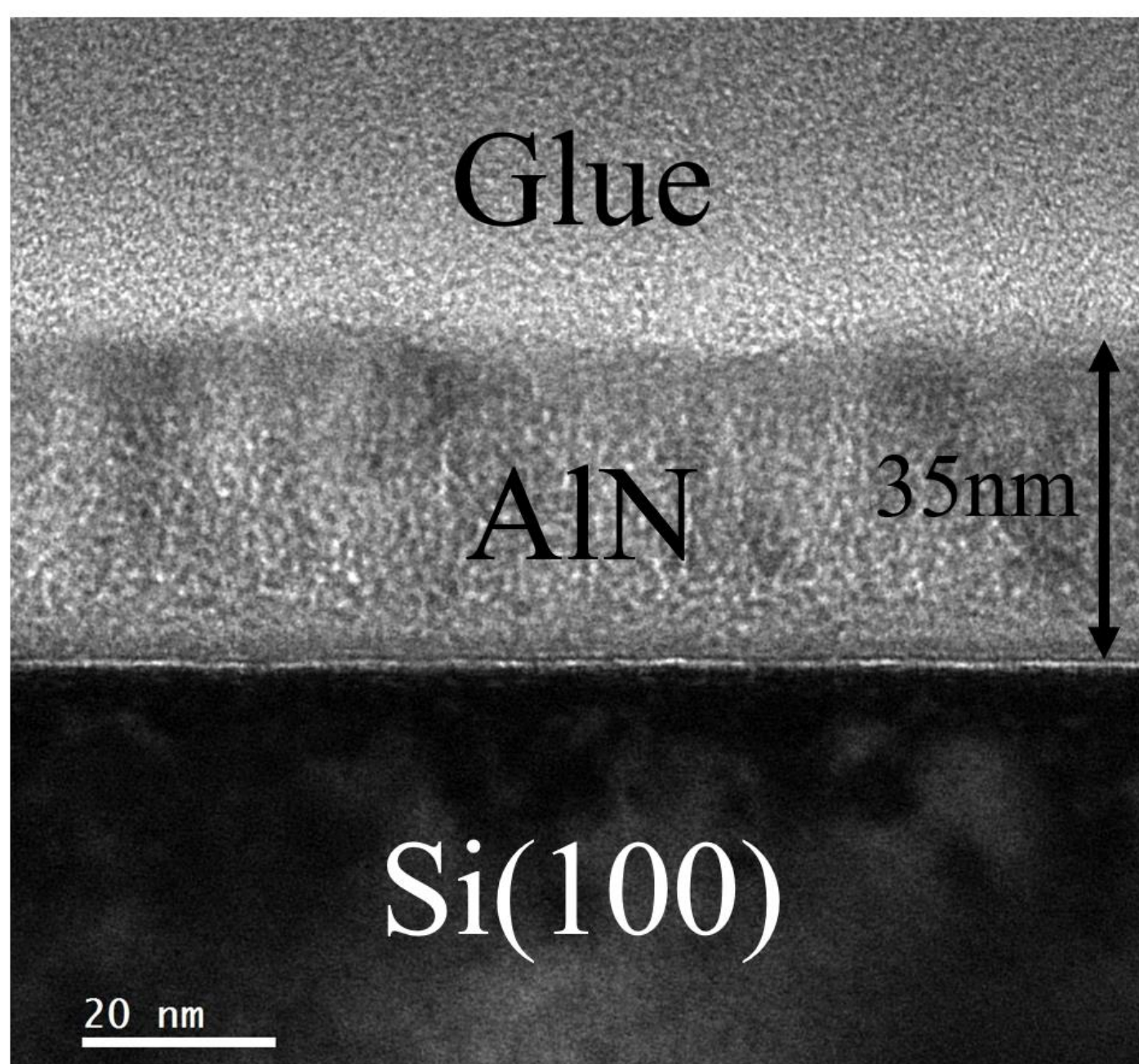
Figure 2. TEM image of ALD AlN film on Si(100).
