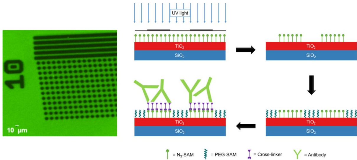
Figure 1. A schematic illustration of the dual SAM patterning procedure (right). After covalent binding of fluorescently labelled antibodies the patterns can be observed with a fluorescence microscope (left).
