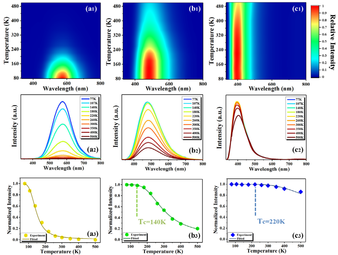
Figure 2. Temperature-dependent PL spectra from 77 to 500K for ZnO QDs with an emitting wavelength of (a) 580 nm, (b) 475 nm and (c) 395 nm.
