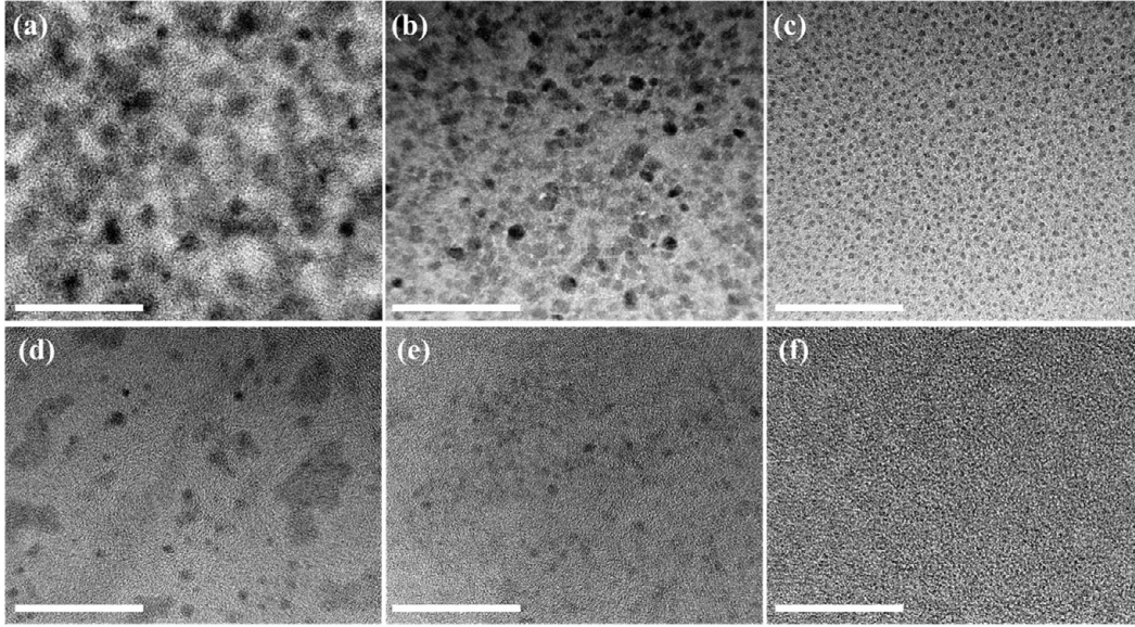
Figure 1. Plan-view of ZnO QDs with surface pretreatment by transmission electron microscopy (TEM), with a DEZn exposure time of (a) 0.03s, (b) 0.02s and (c) 0.01s; (d)-(f) show ZnO QDs having the same growth parameters as those in (a)-(c) but without surface pretreatment. Scale bars are 50 nm.
