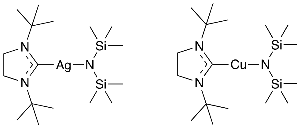
Figure 1: Molecular structure of 1,3 di-tert-butyl-imidazolin-2-ylidene silver(I) 1,1,1-trimethyl-N-(trimethylsilyl) silanaminide [(\text{NHC})\text{Ag}(\text{hmds})] (left) and 1,3 di-tert-butyl-imidazolin-2-ylidene copper(I) 1,1,1-trimethyl-N-(trimethylsilyl) silanaminide [(\text{NHC})\text{Cu}(\text{hmds})] (right). [1]
