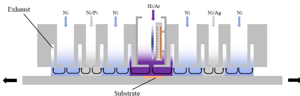
Figure 2: Schematic of Plasma Enhanced Spatial ALD System.
