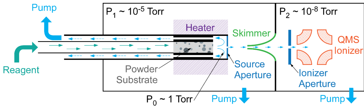
FIGURE 1. Schematic of the ALE-QMS chamber with line of site between sample and ionizer.
