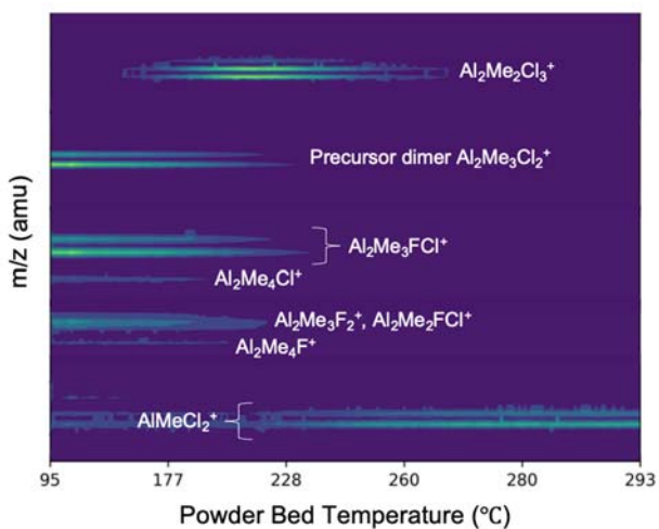
FIGURE 2. Volatile etch products as a function of temperature for the reaction of \text{AlF}_3 with DMAC.
