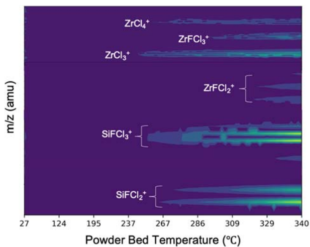
FIGURE 3. Volatile etch products as a function of temperature for the reaction of \text{ZrF}_4 with \text{SiCl}_4 .
