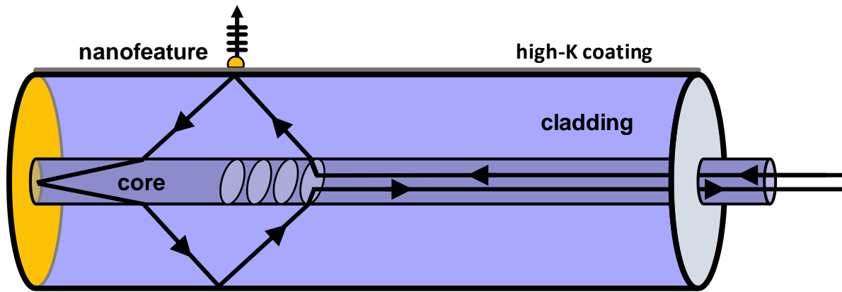
Figure 1: TFBG with Gold Nanofeature
