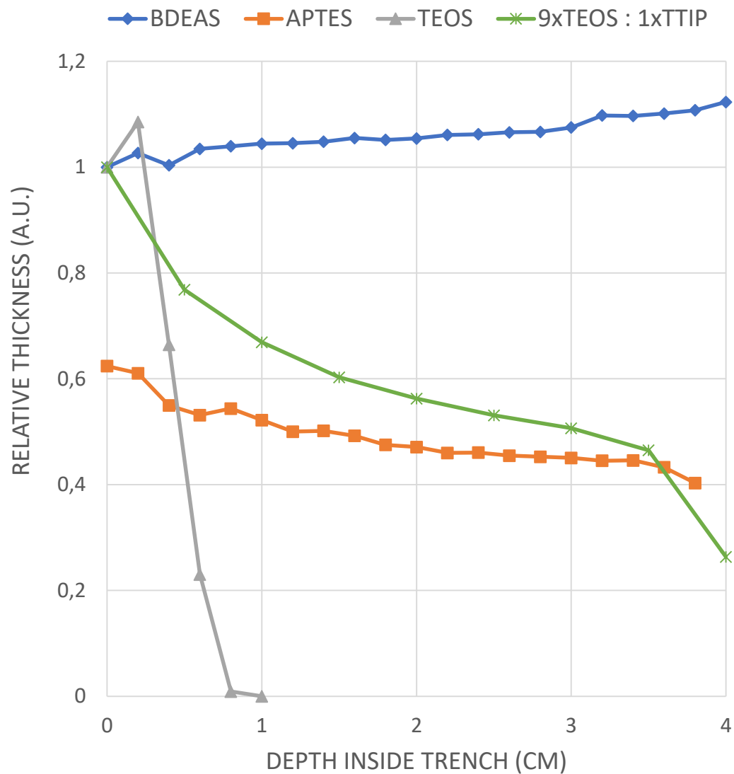
Figure 1: Conformality inside a macroscopic trench for pure and doped \text{SiO}_2 from BDEAS, APTES, TEOS and TEOS+TTIP (9:1 ratio). A relative thickness of 1 corresponds to the thickness on the flat substrate part outside the trench.
