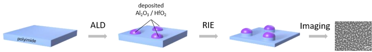
Figure 1. Schematic representation of the proposed qualitative method.
