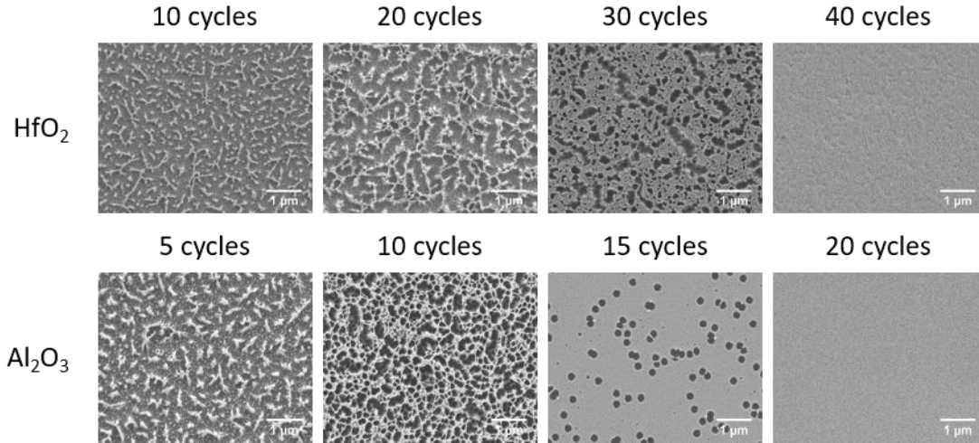
Figure 2. FEG SEM images of the nucleation and closing of a layer of \text{HfO}_2 and \text{Al}_2\text{O}_3 ALD on PI.
