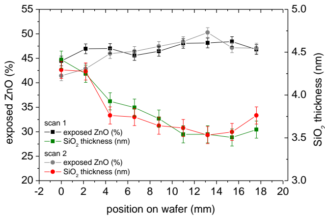
Figure 1. Fraction of exposed ZnO substrate after 110 cycles of SiO 2 deposition (left scale) and average SiO 2 layer thickness (right scale), as a function of wafer position. Two line scans were performed side-by-side to check for repeatability.
