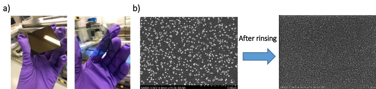
Figure 1. a) Deposited polymer samples on silicon and glass substrates. b) SEM images taken before and after the post-treatment.
