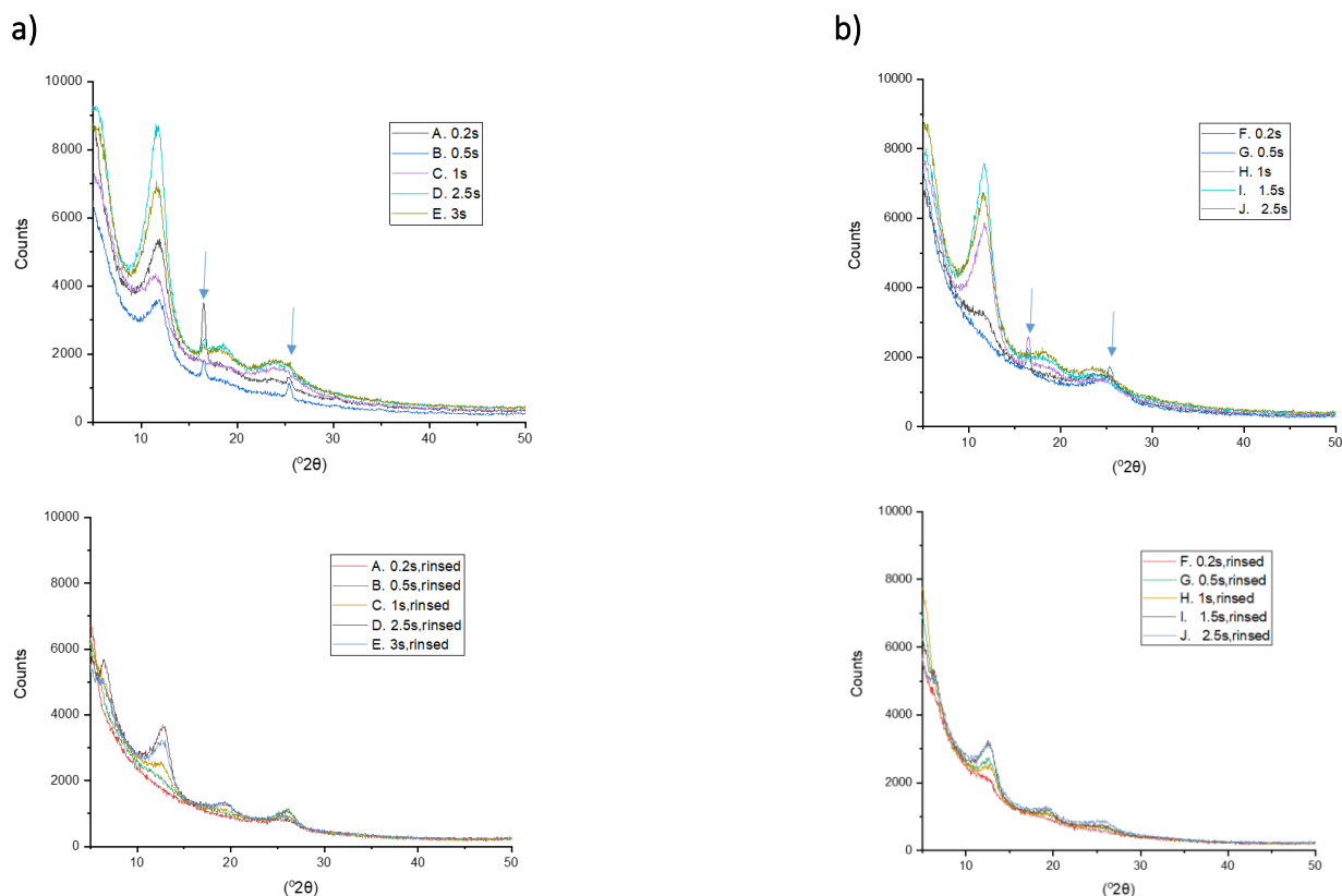
Figure 2. a) X-ray diffractograms of the samples with different \text{ReCl}_5 pulsing durations before and after rinsing them with deionised water. b) X-ray diffractograms of the samples with different EDOT pulsing durations before and after rinsing them with deionized water. (Rhenium oxychloride reflections disappeared in the post-treated samples.)
