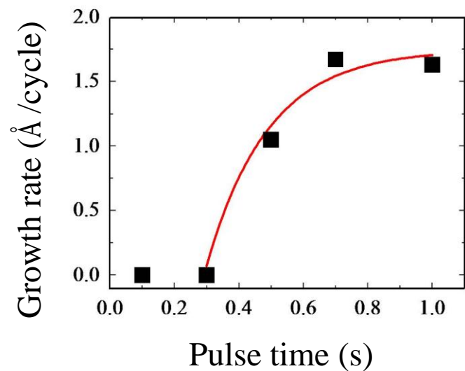
Fig.1. The growth rate of SnO 2 versus TDMASn pulse time.
