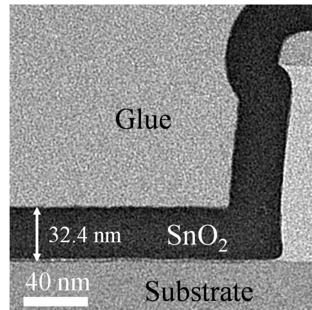
Fig. 3. Cross-sectional TEM image of SnO 2 thin film (the scale bar is 40 nm).
