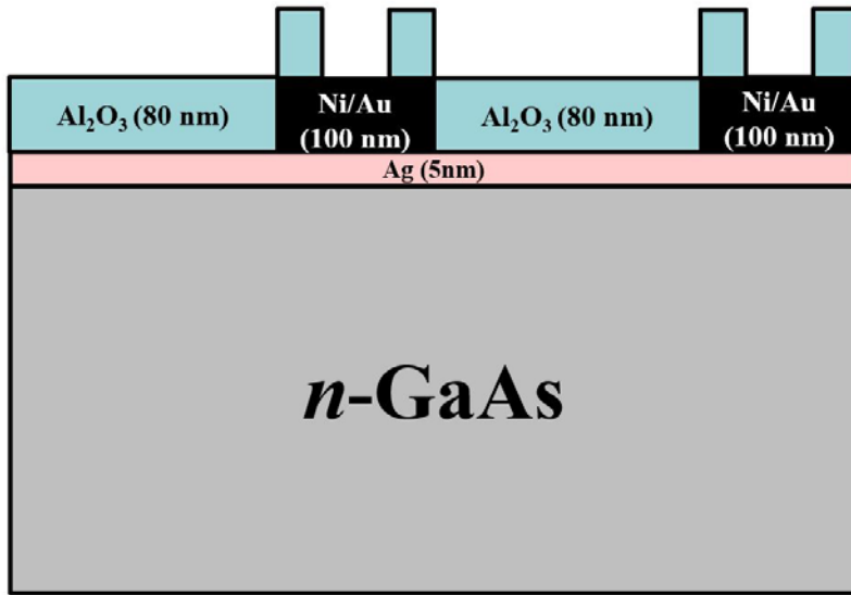
Figure 1. Schematic structure of Ag/n-GaAs Schottky junction solar cell with 80 nm ALD-grown Al 2 O 3 ARC layer
