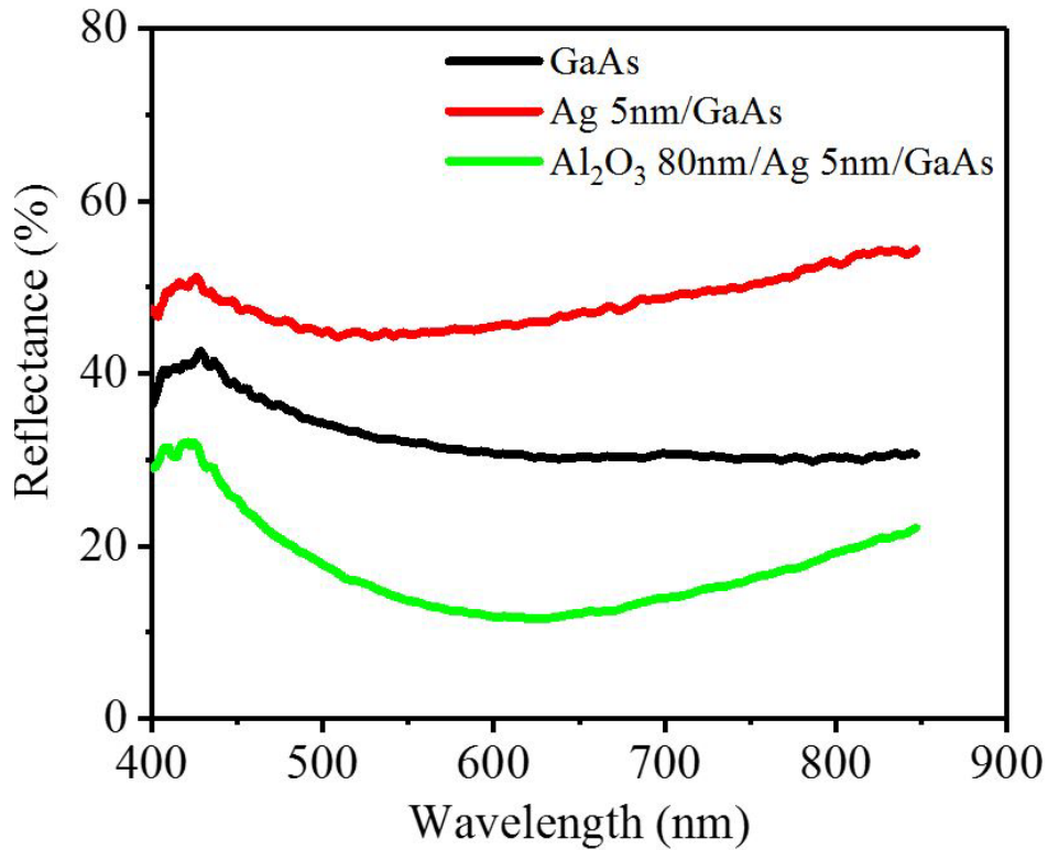
Figure 2. Reflectance measurements from the top surface of M-S Schottky structure before and after deposition of 80 nm Al 2 O 3 ARC layer
