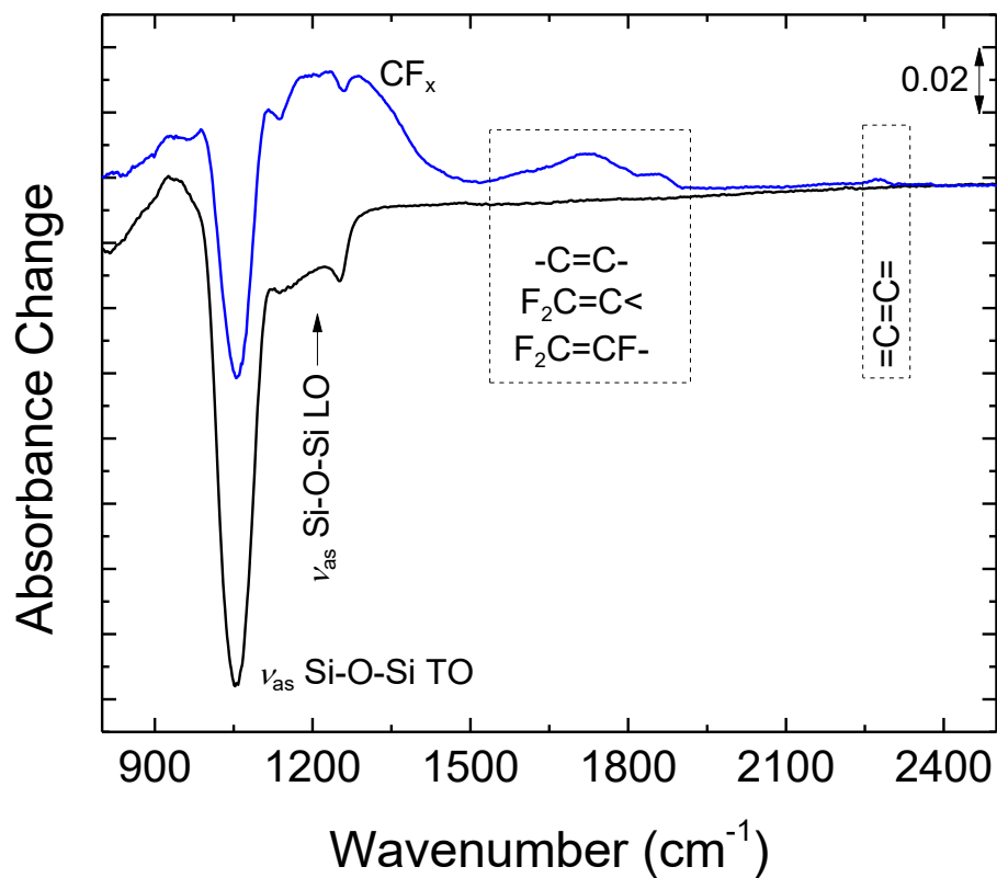
Figure 1: Infrared absorbance change for 5 cycles of ALE on a bare SiO 2 film (black spectrum) and the prefunctionalized SiO 2 film (blue spectrum). The reference spectrum was taken immediately prior to the first CF x deposition half-cycle for both spectra.
