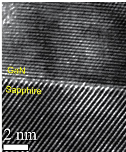
Figure 2. Cross-sectional HRTEM image of the GaN epilayer grown by ALAE.
