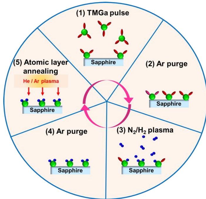
Figure 1. The schematic diagram of the processing cycle of the atomic layer annealing and epitaxy (ALAE) technique.
