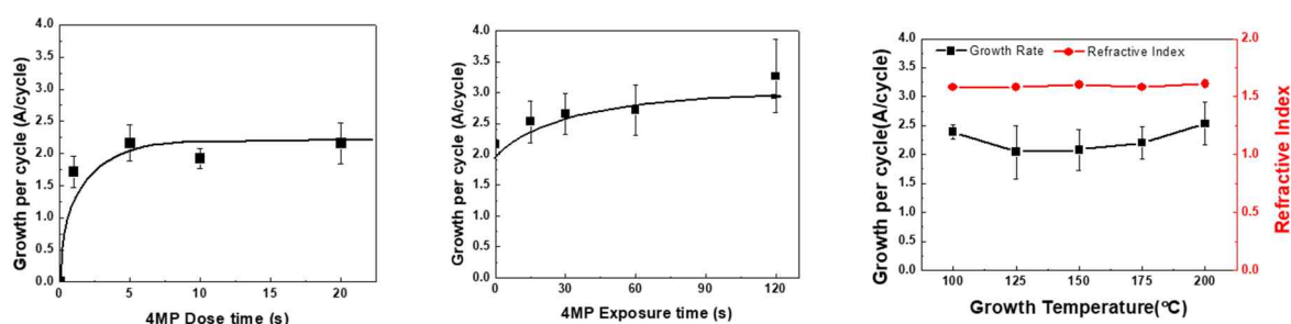
Figure 1 Growth of alucone 4MP dose time(left), exposure time(middle), growth temperature(right) dependence
