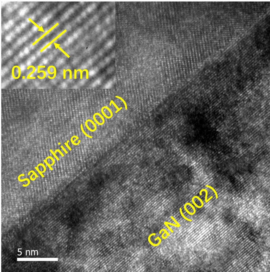
HR-TEM image of ~20 nm GaN grown at 350 °C on sapphire (0001) substrate. Inset image shows the as-grown GaN displays a single hexagonal (002) phase.
