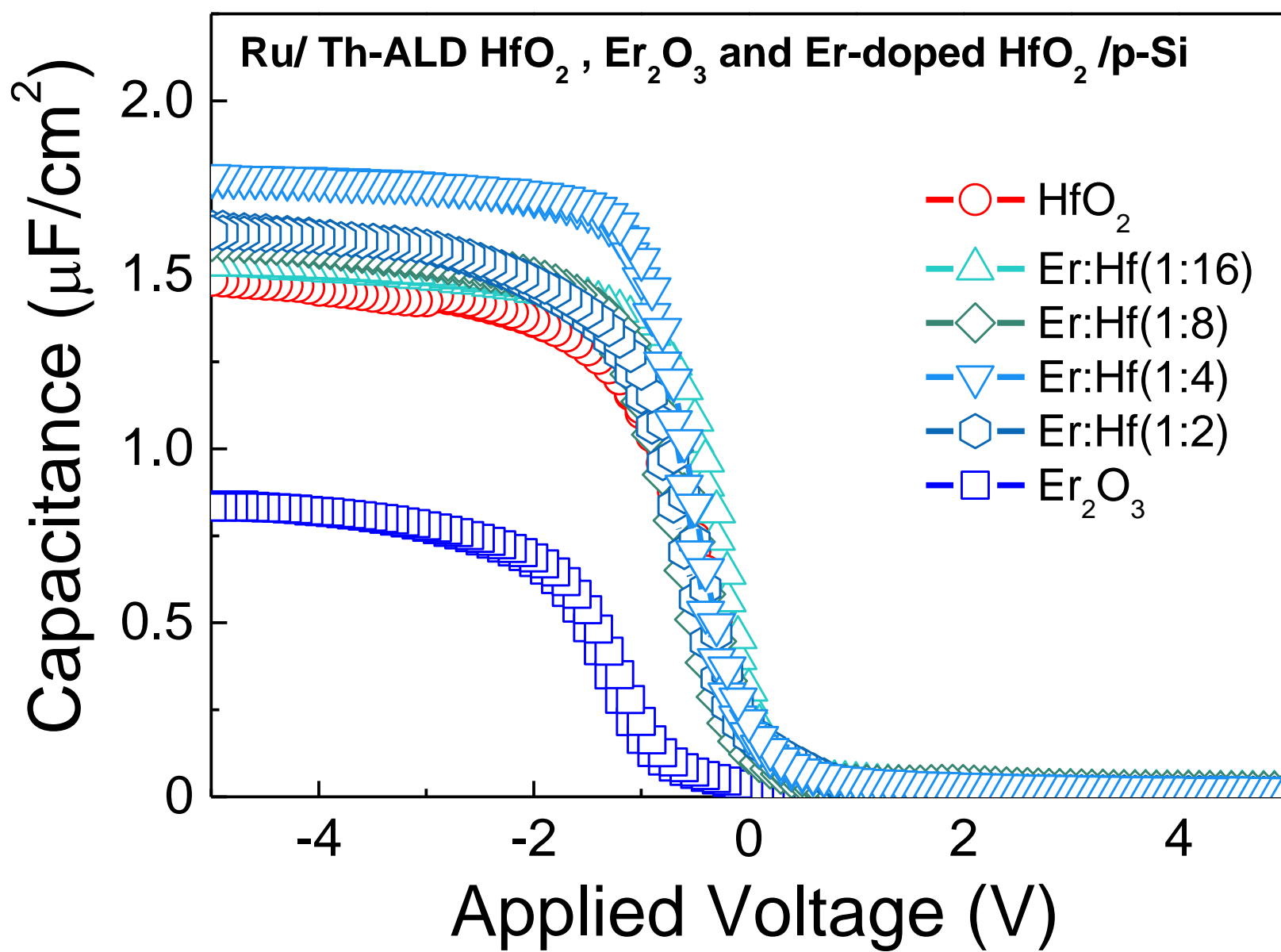
Figure2. C-V curves of MOS capacitors with ALD \text{HfO}_2 and Er-doped \text{HfO}_2 films with varying compositions.
