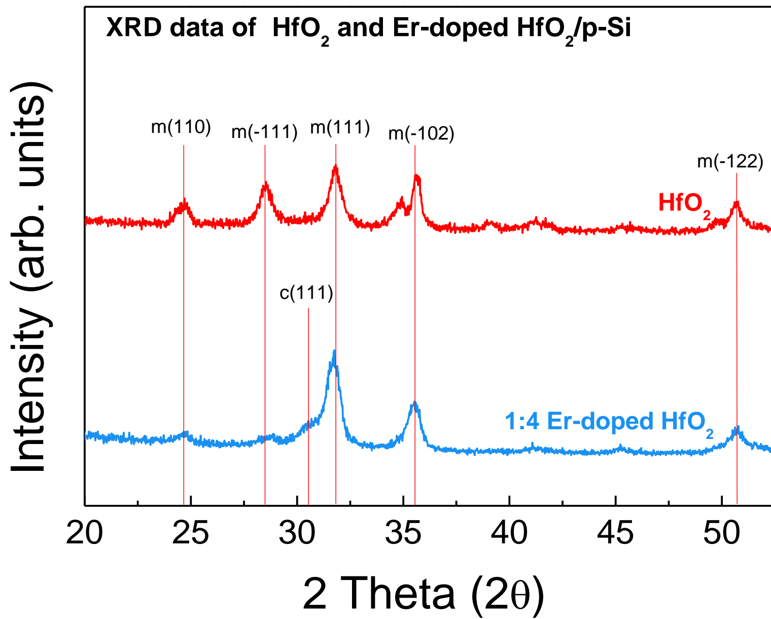
Figure1. XRD results of ALD \text{HfO}_2 and 1:4 Er-doped \text{HfO}_2 films.
