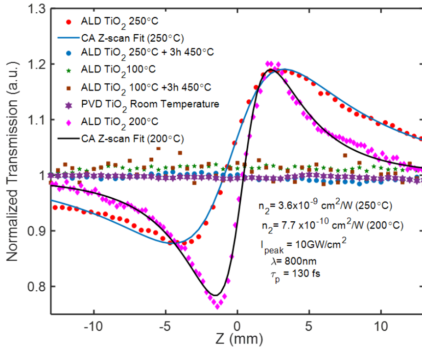
Figure 1. Z-scan results for ALD TiO 2 (100, 250°C) and PVD TiO 2 films
