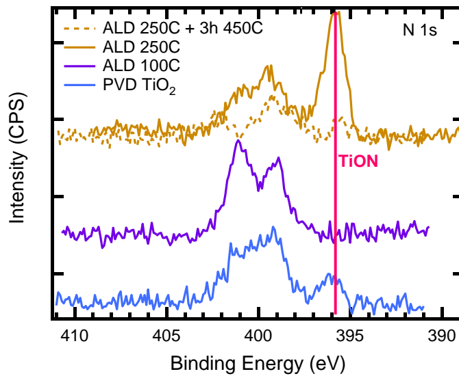
Figure 2. XPS results for some of the films shown in Figure 1. The high nonlinear response in some of the films is linked to the presence of a small at. % of TiN bonding.
