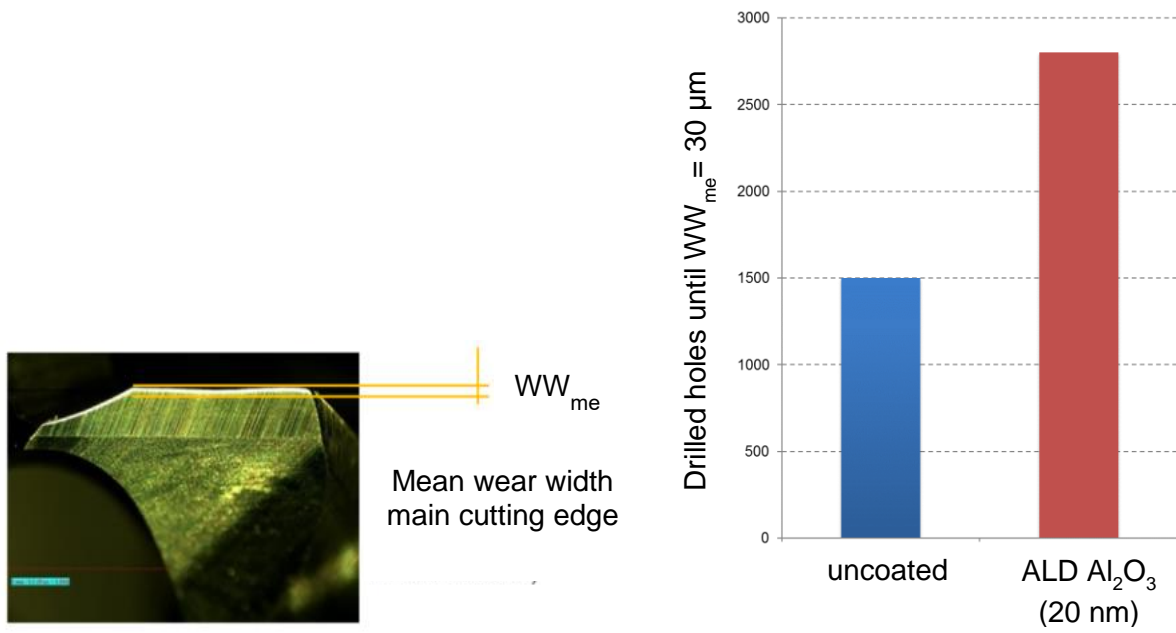
Figure 1: left shows a coated drill from the top with a marking for the width of the main cutting edge; right shows the number of drilled holes for with 20 nm Al_2O_3 coated tools in comparison to uncoated tools until the width of the main cutting edge reaches 30 \mu m
