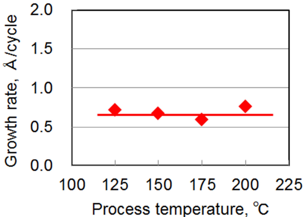
Fig.2: ALD growth rate of gallium oxide film on Si substrate using GNP-7 & H 2 O.
