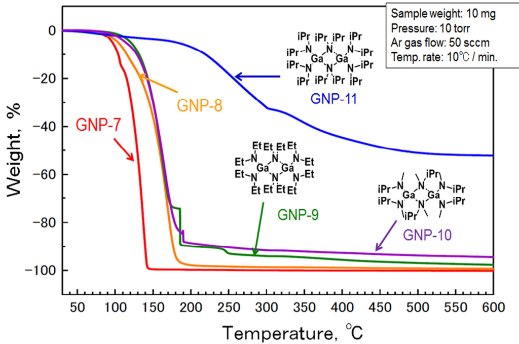
Fig.1: TGA spectra of various kinds of N-based gallium molecules including GNP-7 (under 10 torr)
