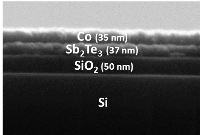
Figure 1: SEM figure cross-sectional view image of a Co/Sb 2 Te 3 heterostructure deposited on a SiO 2 /Si substrate.
