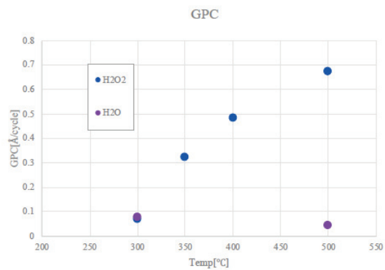
Figure 2. SiO 2 Growth Per Cycle (GPC), H 2 O 2 /H 2 O vs H 2 O.
