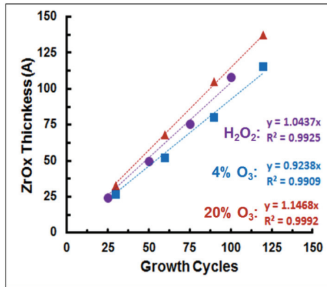
Figure 1. Growth curve for ZrO 2 ALD with Anhydrous Hydrogen Peroxide vs 4% and 20% O 3 .
