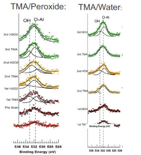
Figure 3. XPS of Al 2 O 3 Nucleation on Si-H: Anhydrous H 2 O 2 vs H 2 O.
