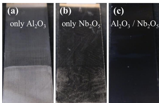
Fig.2 Surface images of SUS304 plates with only alumina, only \text{Nb}_2\text{O}_5 and alumina/ \text{Nb}_2\text{O}_5 films. All the samples were immersed partially in an HCl acid (36 wt%).
