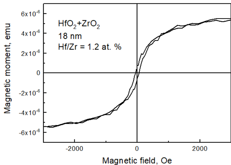
Fig.1 Magnetic moment in a HfO 2 -ZrO 2 nanolaminate on Si(100) substrate with respect to external magnetic field, measured by vibrating sample magnetometer, on the left panel. Polarization charge – applied electric field curve for the same sample on TiN on the right panel.
