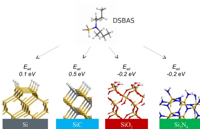
Figure 1. Di(sec-butylamino)silane (DSBAS) precursor reacting with different Si-based surfaces (Si:H, SiC:H, SiO 2 :OH and Si 3 N 4 :NH 2 /NH). DSBAS reacts selectively with SiO 2 and SiN x but not with Si and SiC surfaces.
