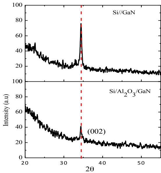
Fig. 1 XRD pattern of the Si/GaN and Si/Al 2 O 3 /GaN heterostructures ,
