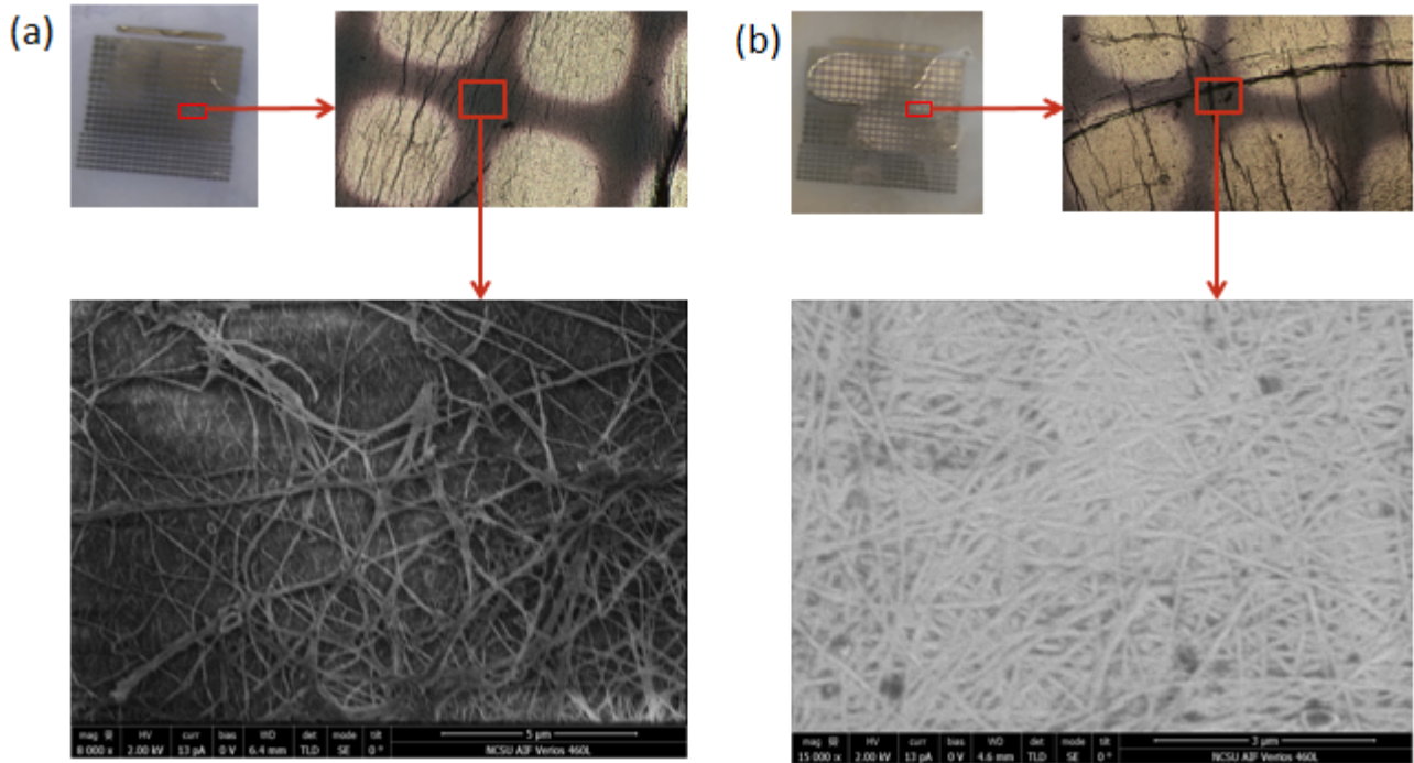
Fig 1. Optical microscope and SEM images a) before ALD deposition b) after ALD deposition
