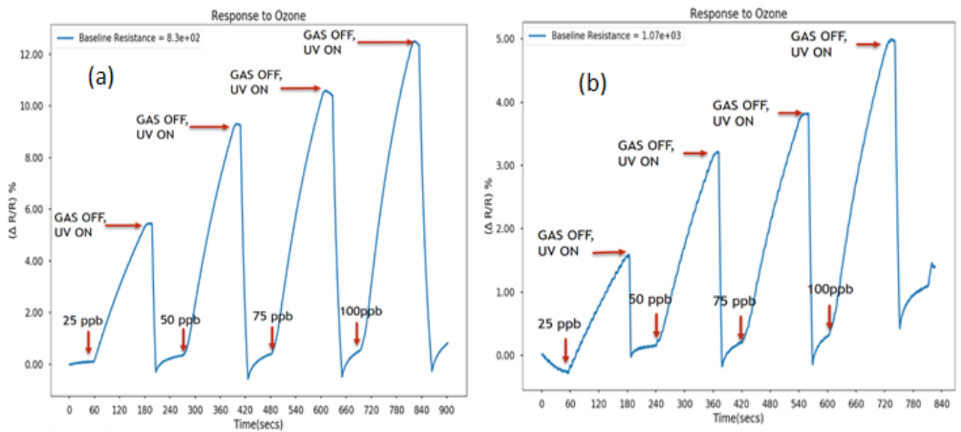
Fig 2. Response from (a) Nanocellulose substrate sensor (b) Silicon substrate sensor, to ozone in the 25 to 100ppb concentration range with UV recovery for resetting to baseline resistance.
